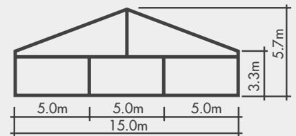
Type: ET15/330
