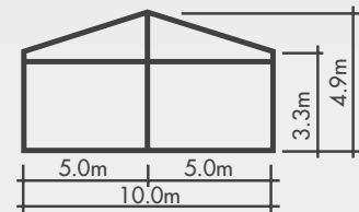
Type: ET10/330
