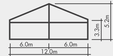
Type: ET12/330
